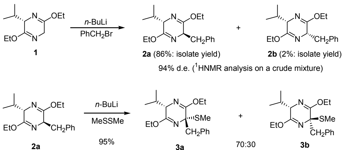
Scheme 2. Benzylation of Schöllkopf's bislactim ether 1 and methylsulfanylation of major product 2a
