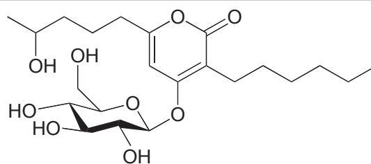
whitmanoside A
