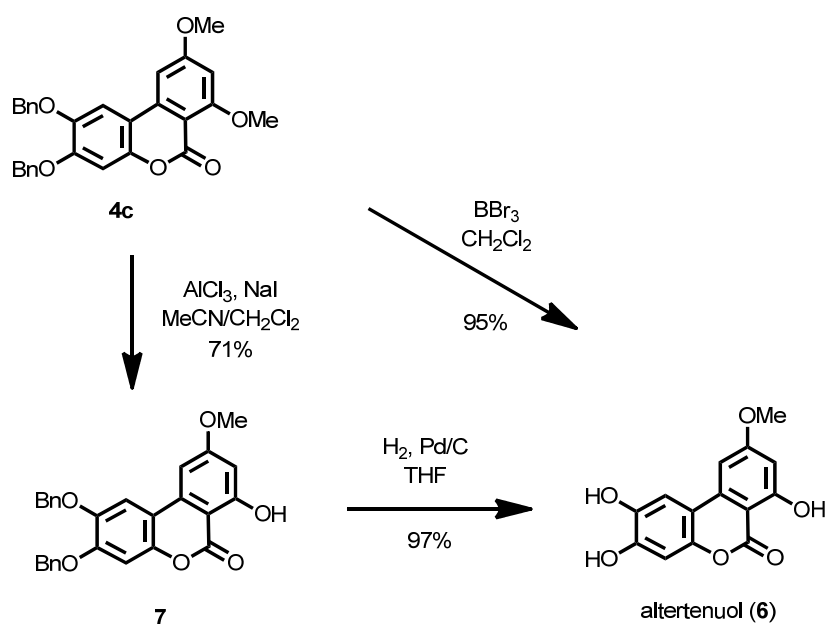
Scheme 1. Transformation of 4c into Alternenuol ( 6 )
