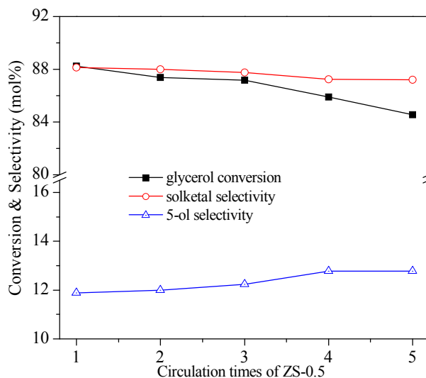
Figure 1S. Results of cycle utilization of ZS-0.5 catalyst in the glycerol ketalization with acetone
