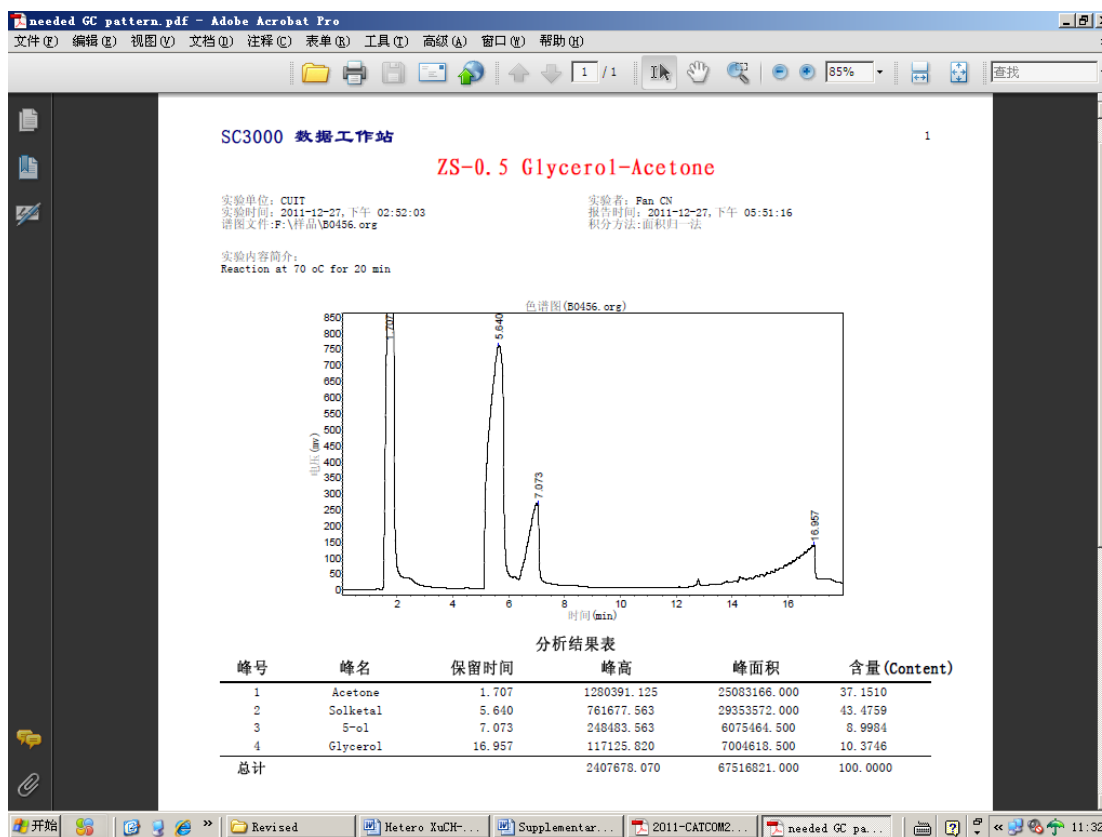
Figure 2S. GC analysis results of liquid samples from glycerol ketalization with acetone over ZS-0.5 at 70 °C for 20 min
