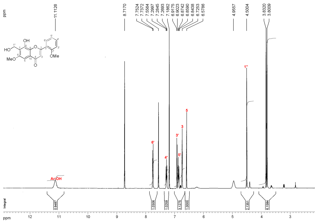
Figure S6. 1 H NMR spectrum of compound 2
