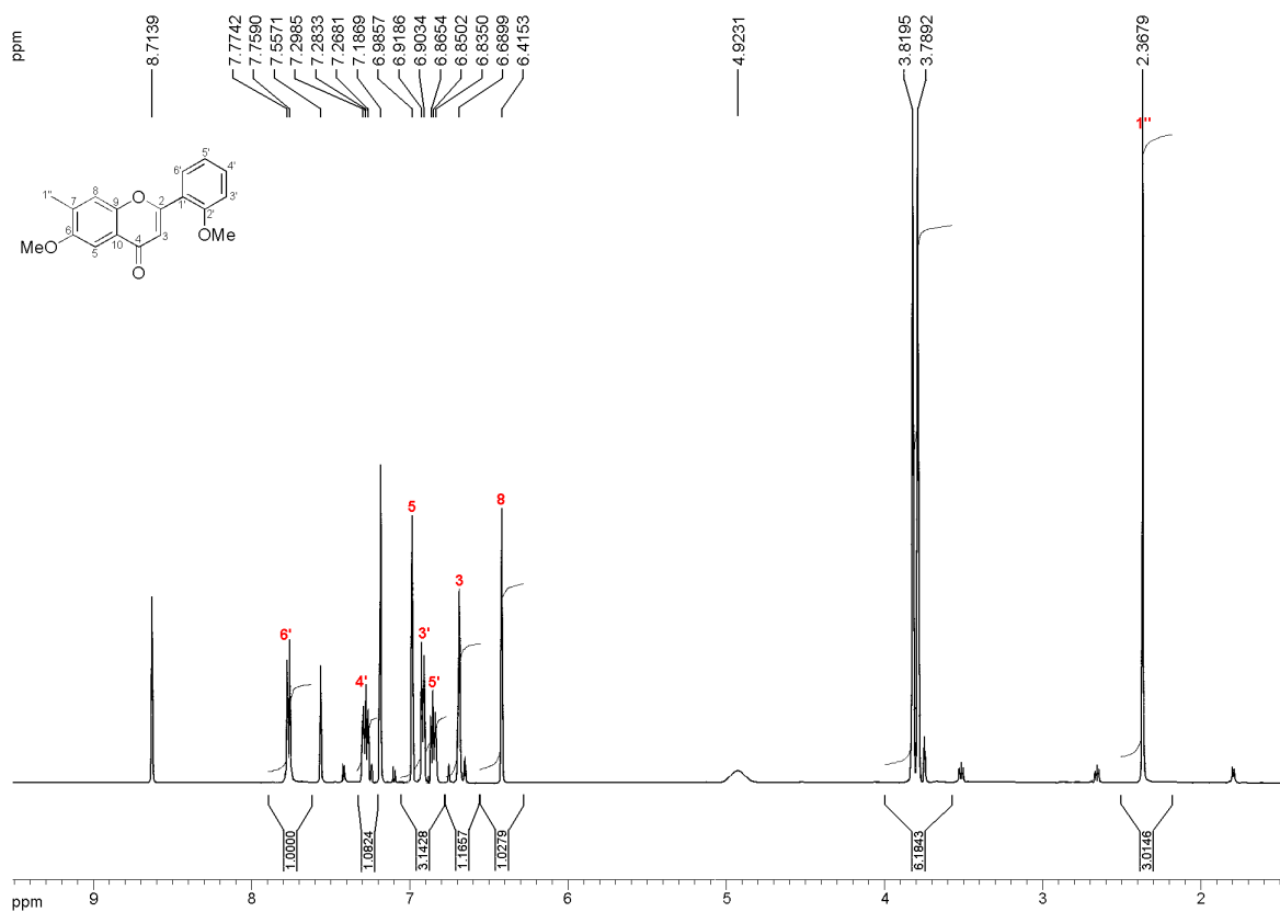
Figure S8. 1 H NMR spectrum of compound 3
