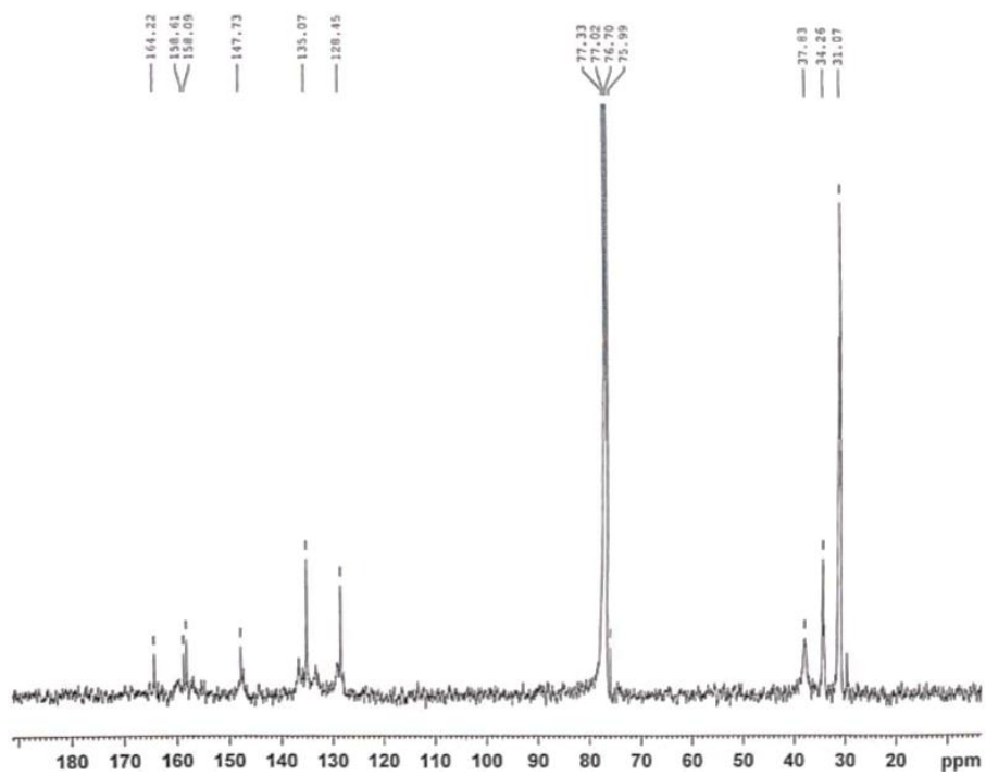
Figure S7: ^{13}\text{C} NMR spectrum of compound 4a
