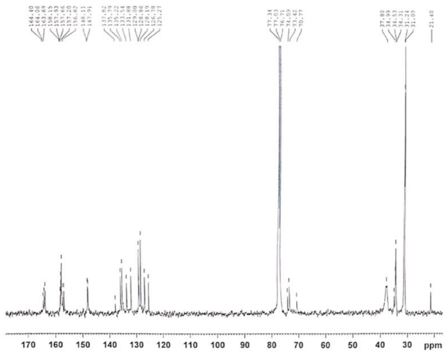
Figure S8: ^{13}\text{C} NMR spectrum of compound 4b
