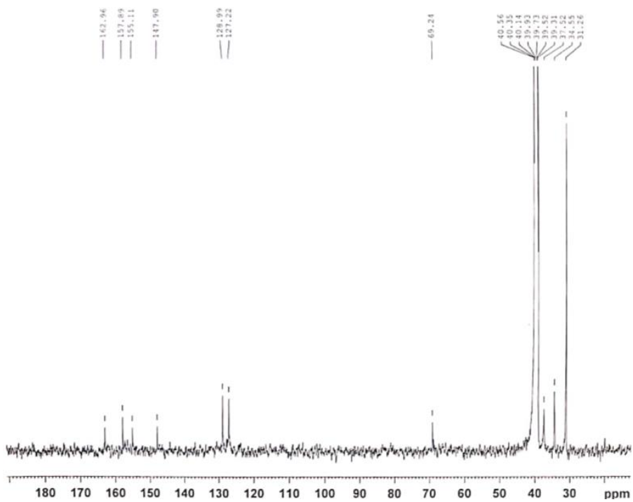
Figure S9: 13 C NMR spectrum of compound 4c
