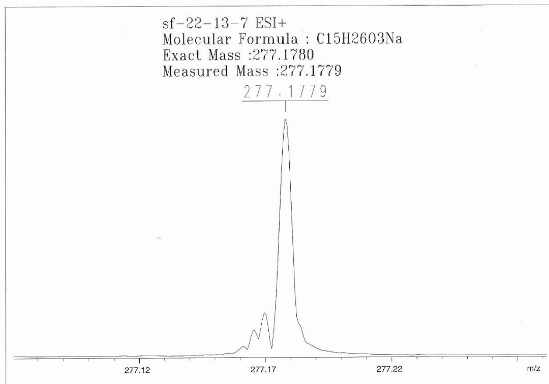
S1. ESIMS spectrum of compound 1
