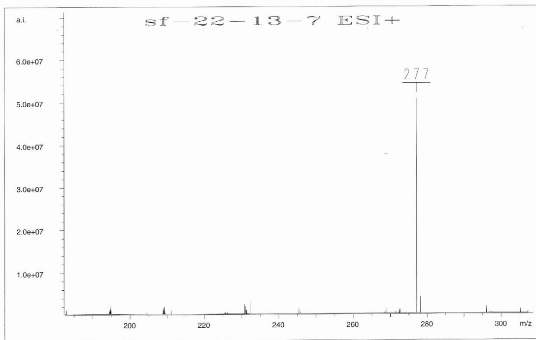
S1. ESIMS spectrum of compound 1
