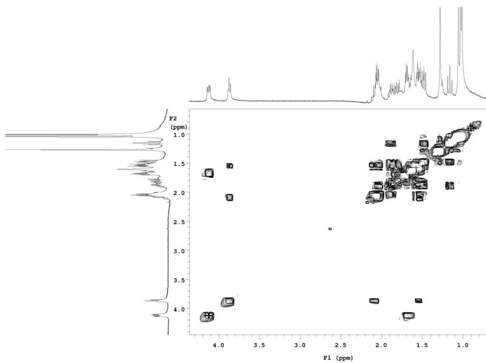
S7. 1 H- 1 H COSY spectrum of compound 1 in CDCl 3
