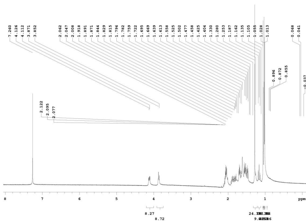
S4. 1 H NMR spectrum (400 MHz) of compound 1 in CDCl 3
