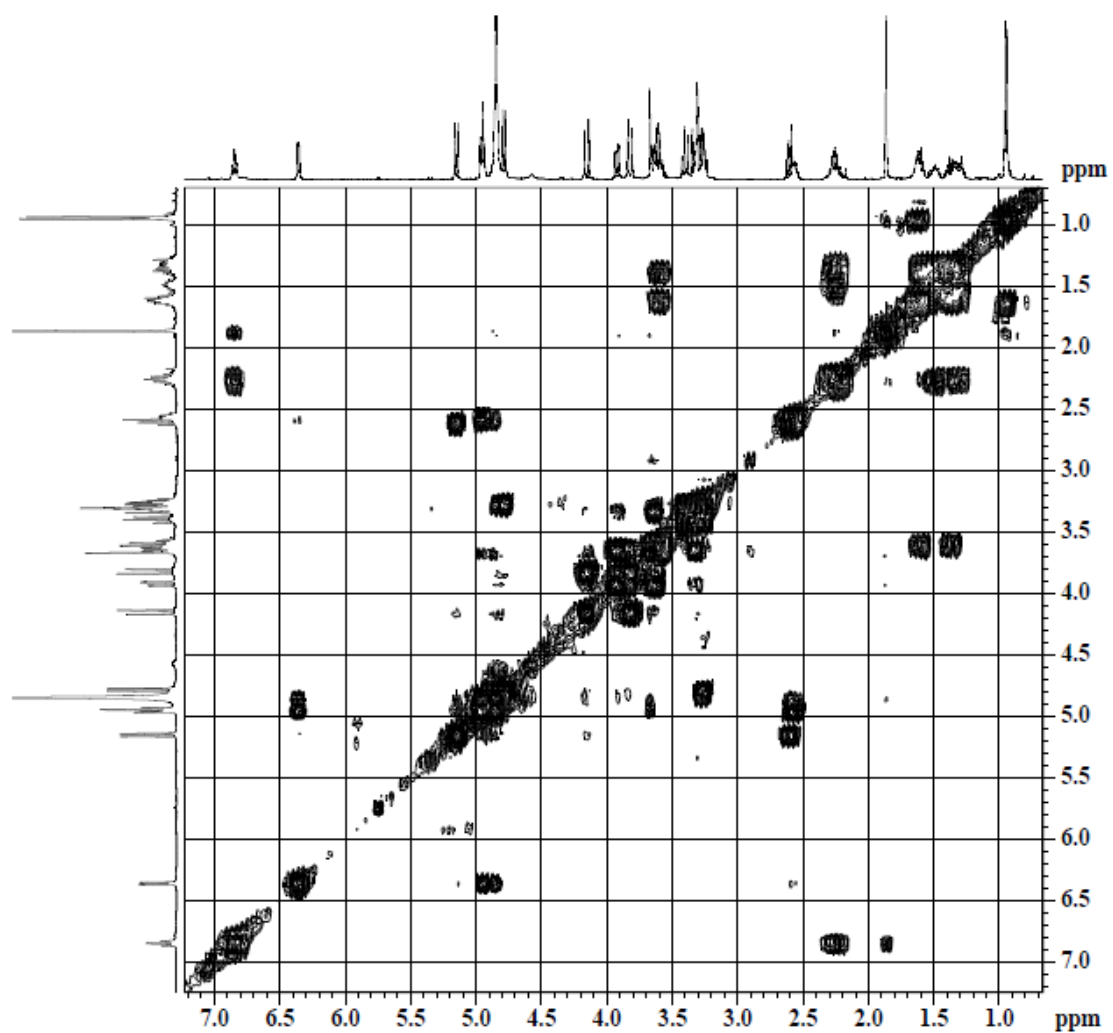
Figure S3 The COSY spectrum of compound 1 in CD 3 OD
