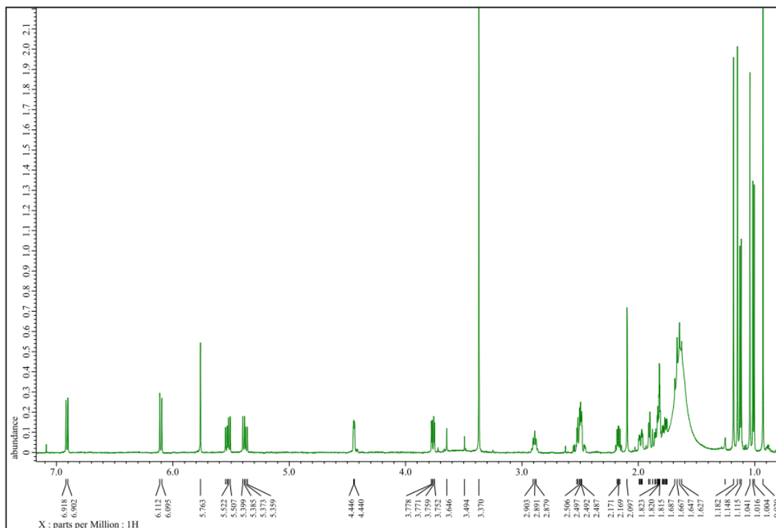
S1. ^1\text{H} NMR spectrum of terreus steroid ( 1 ).
