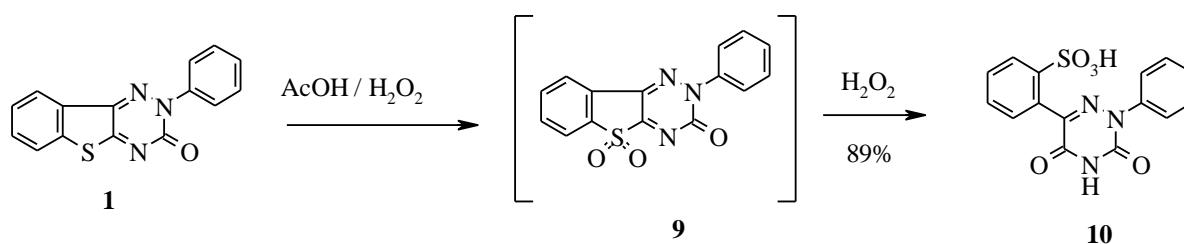
Scheme 4. Oxidative cleavage of 1,2,4-triazine 1 by peracetic acid
