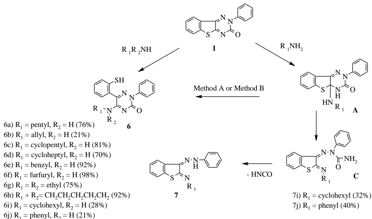
Scheme 3. Reaction mechanism for cleavage of 1,2,4-triazine 1 by N-nucleophiles
