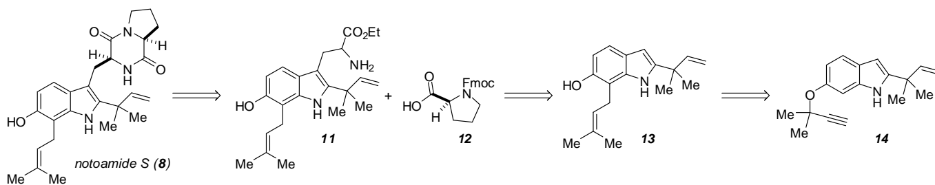
Scheme 3. Retrosynthetic analysis of notoamide S.
