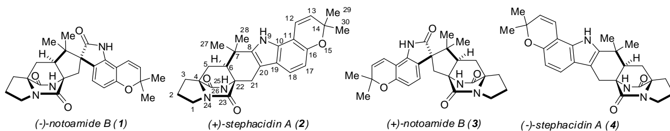
Figure 1. (+) And (–)-stephacidin A and (+) and (–)-notoamide B.
