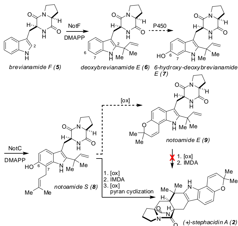
Scheme 1. Proposed biosynthesis of stephacidin A.
