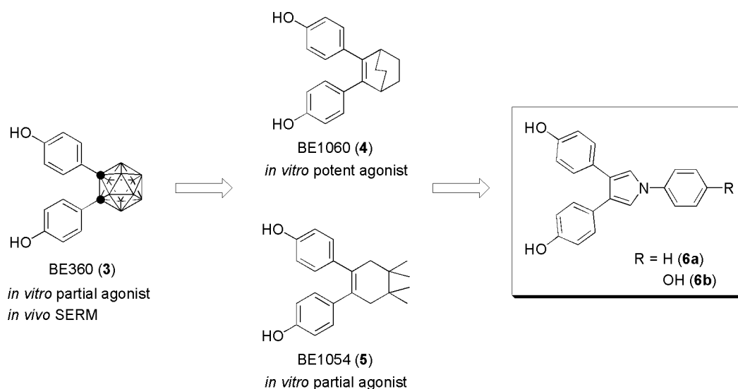
Figure 2. Structures of ER modulators and newly designed ER modulator candidates based on a bisphenol structure.
